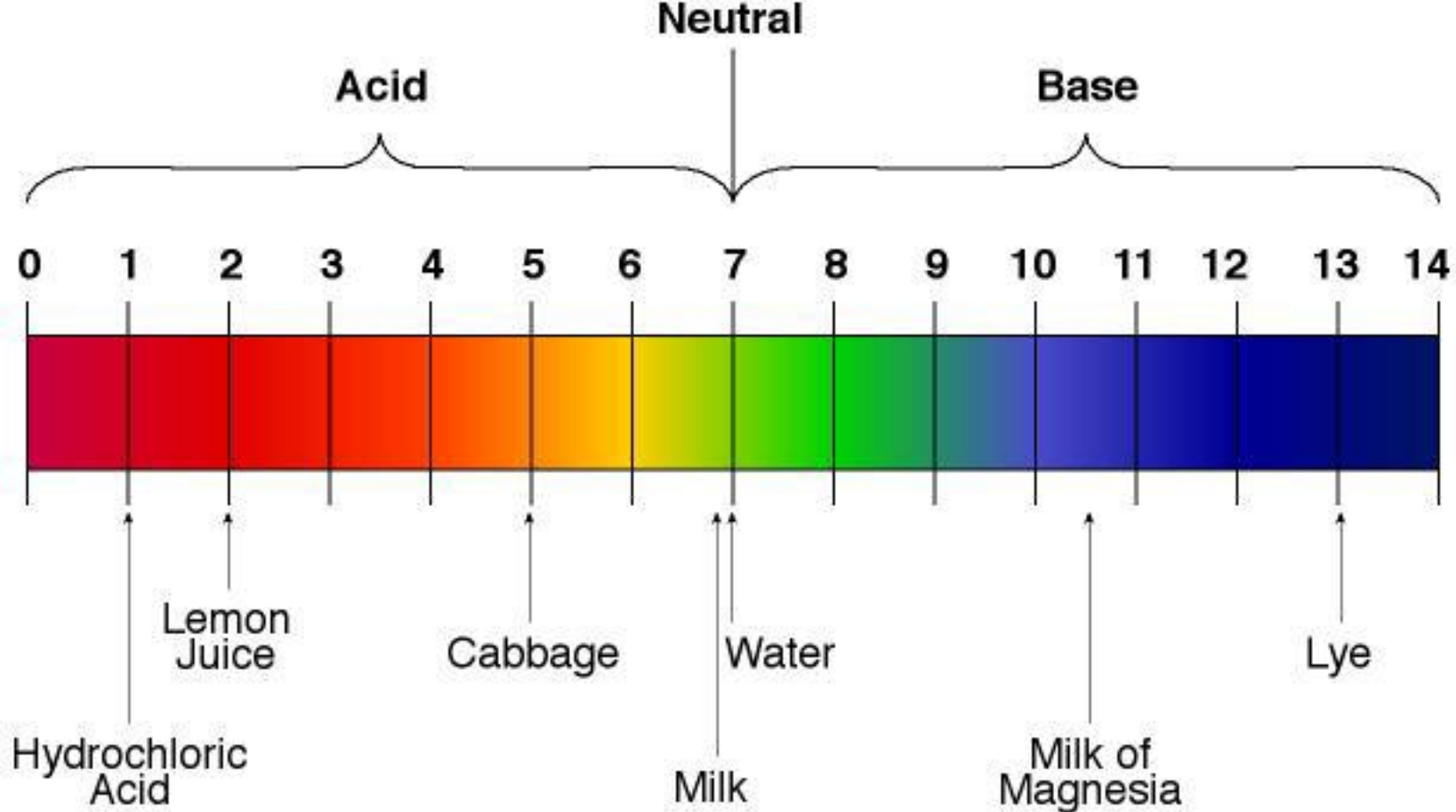
The pH Scale
